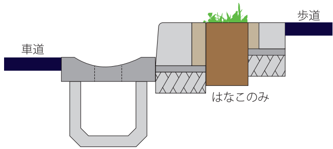
両面土舗装抑え | HKM-020603
