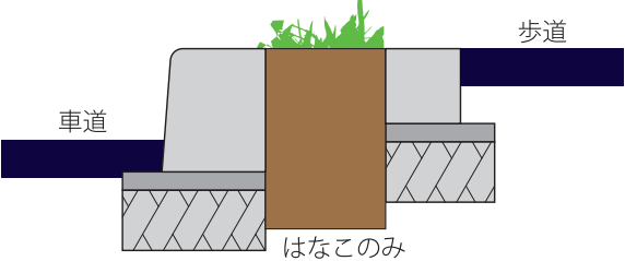
歩車道境界縁石抑え | HKM-030603
